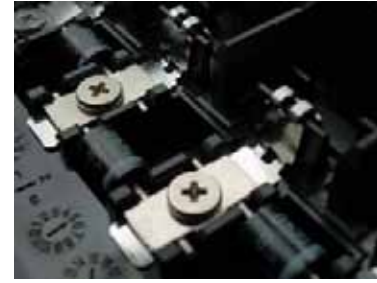
Screw Down Mechanism for In-Field Diode Replacement
